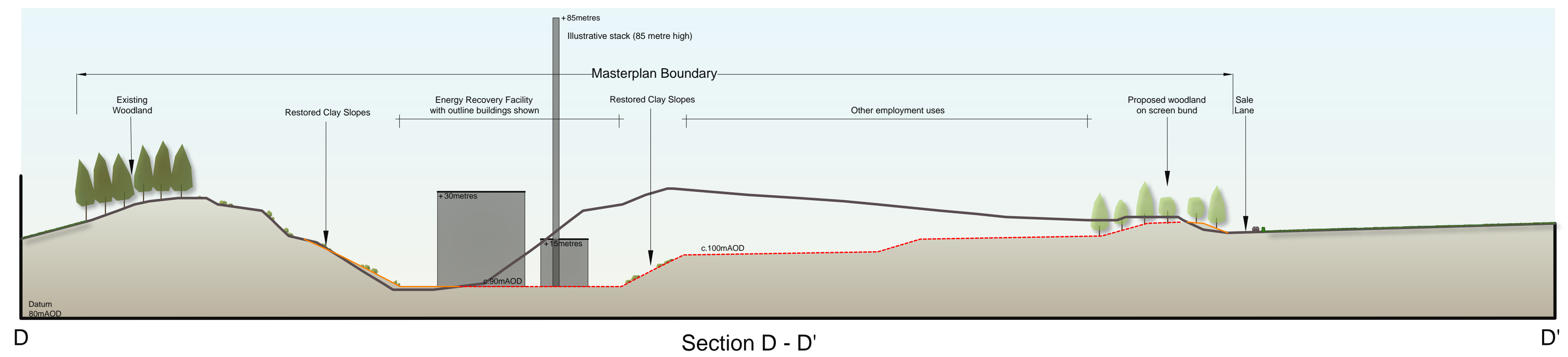
Illustrative Cross Sections Through Buttington Quarry Including Schematic ERF Facility
